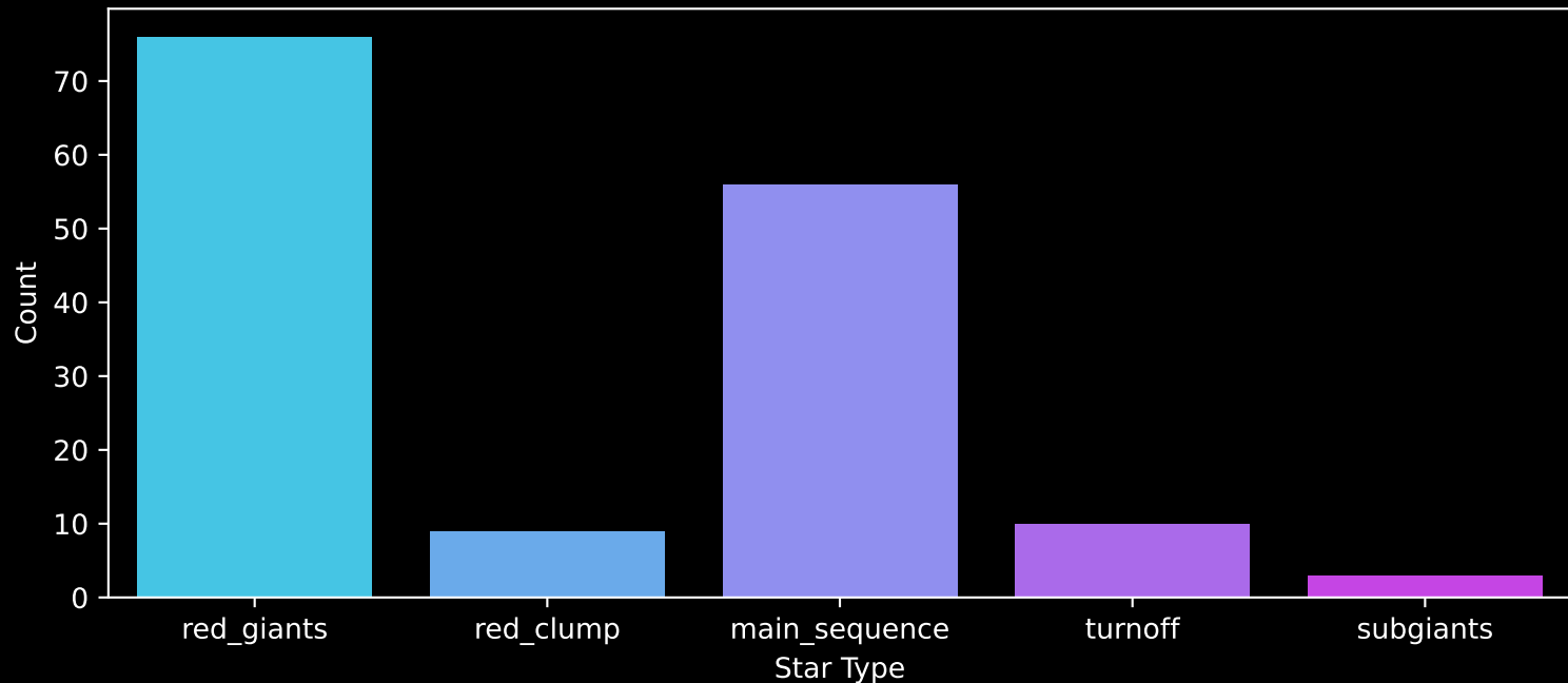
APOGEE DR17 Field: [K2_C7_012-17] Count plot of Star Type
