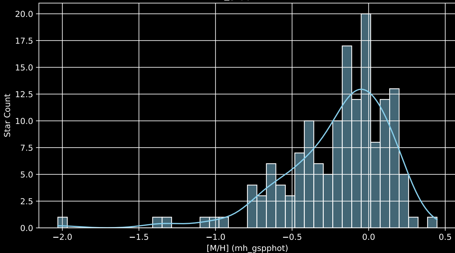
APOGEE DR17 Field: [K2_C7_012-17 [M/H] (mh_gspphot) (n= 153)
