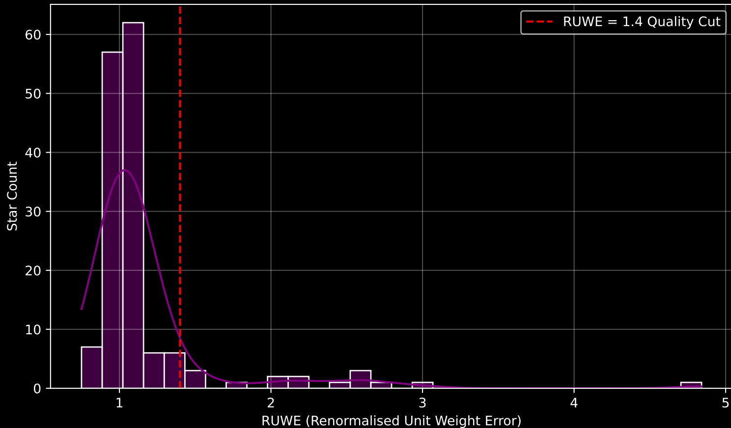
GAPOGEE DR17 Field [K2_C7_012-17] RUWE Distribution (n= 153)
