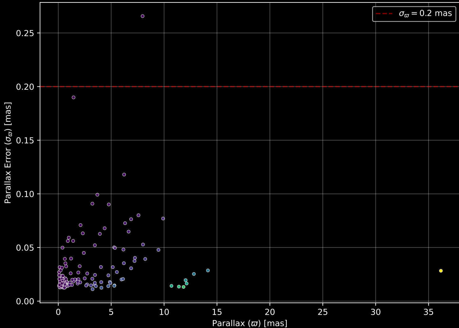
APOGEE DR17 Field: [K2_C7_012-17] Parallax Quality (n= 154)
