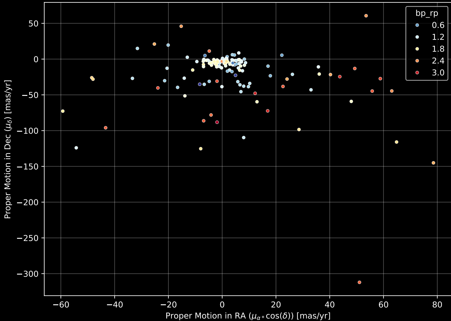
APOGEE DR17 Field: [K2_C7_012-17] Proper Motion Diagram (n= 154)
