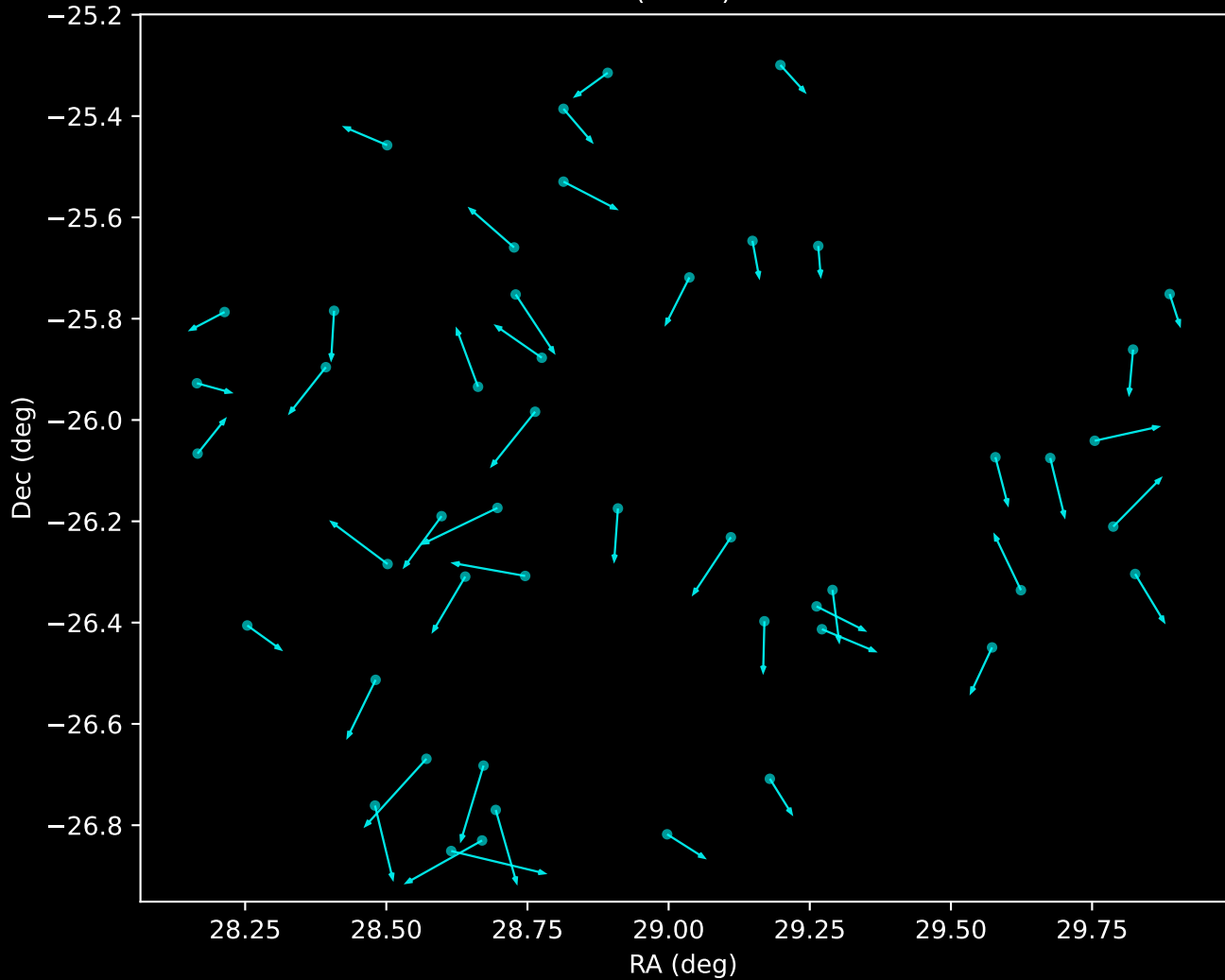
APOGEE DR17 Noise Stream Proper Motion Vectors (n=48)
